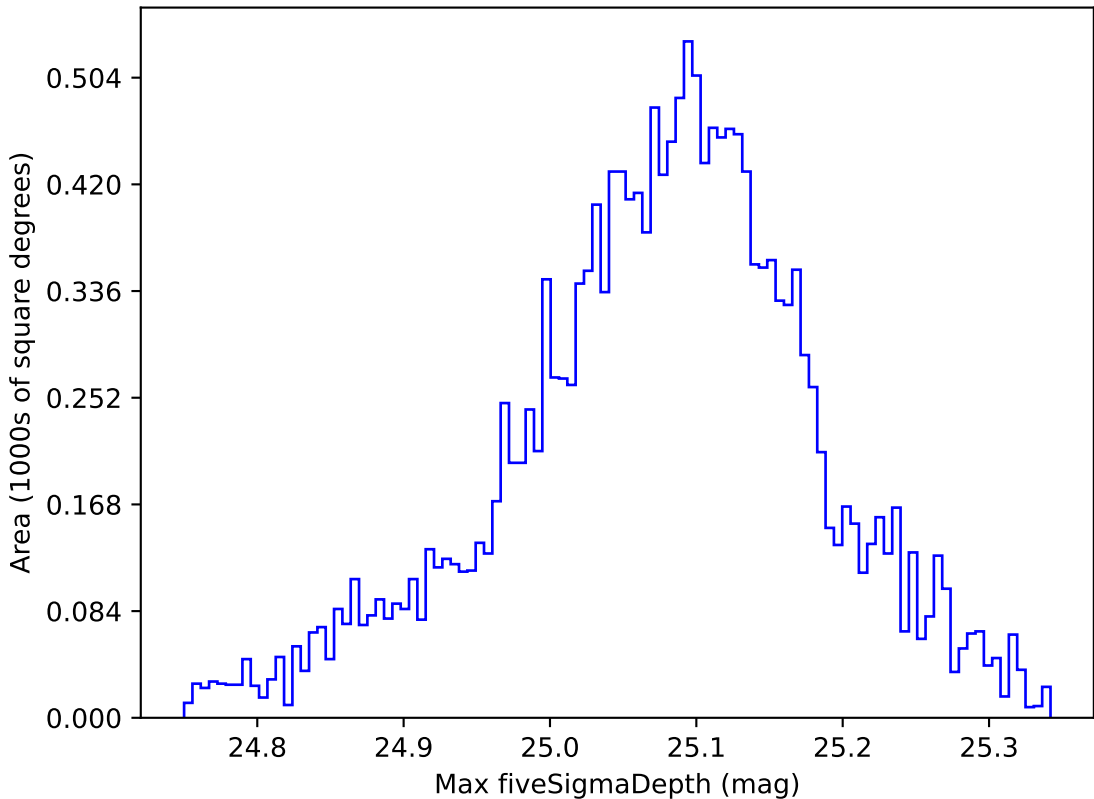
telescope_jerk_v3.5_10yrs WFD all bands: Max fiveSigmaDepth
