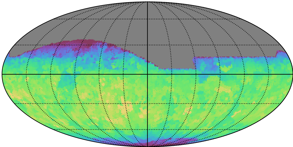
telescope_jerk_v3.5_10yrs All sky z band: Max fiveSigmaDepth
