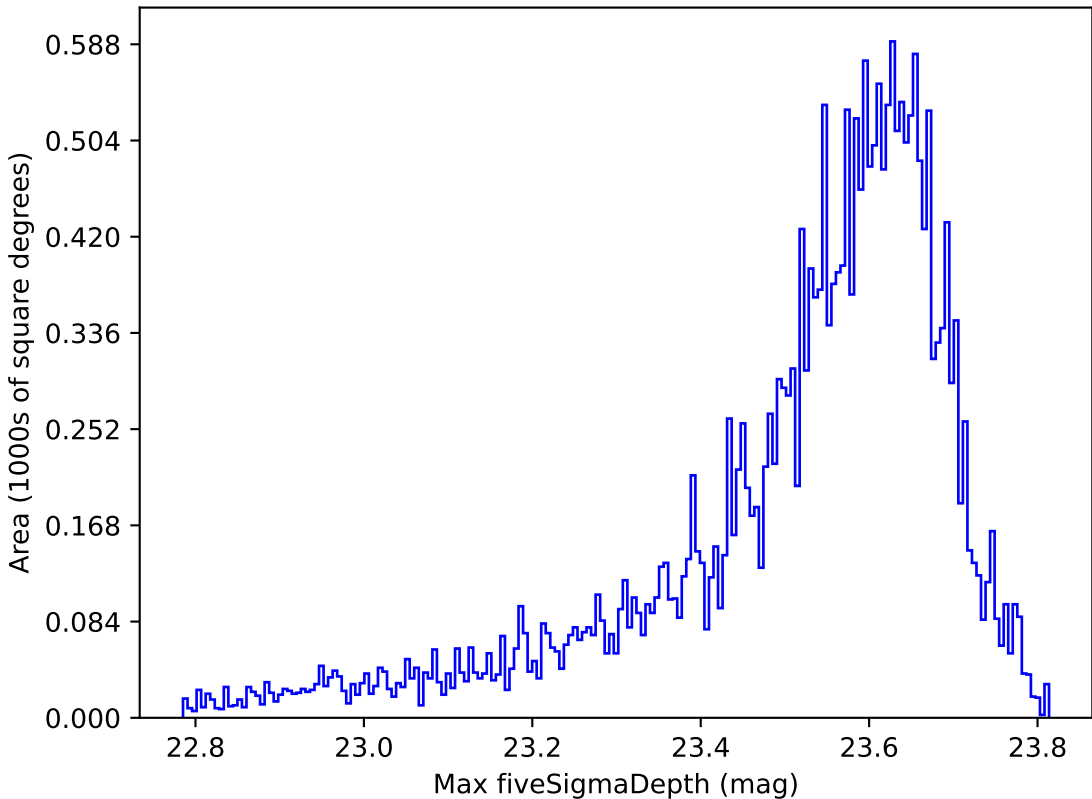
telescope_jerk_v3.5_10yrs All sky z band: Max fiveSigmaDepth
