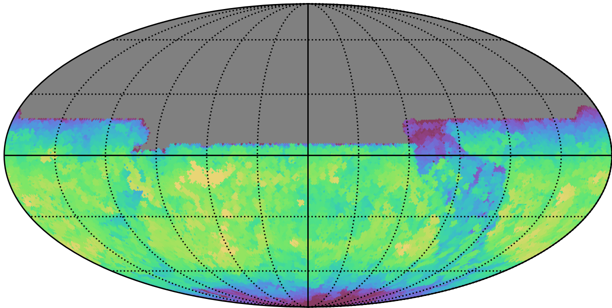
telescope_jerk_v3.5_10yrs All sky y band: Max fiveSigmaDepth
