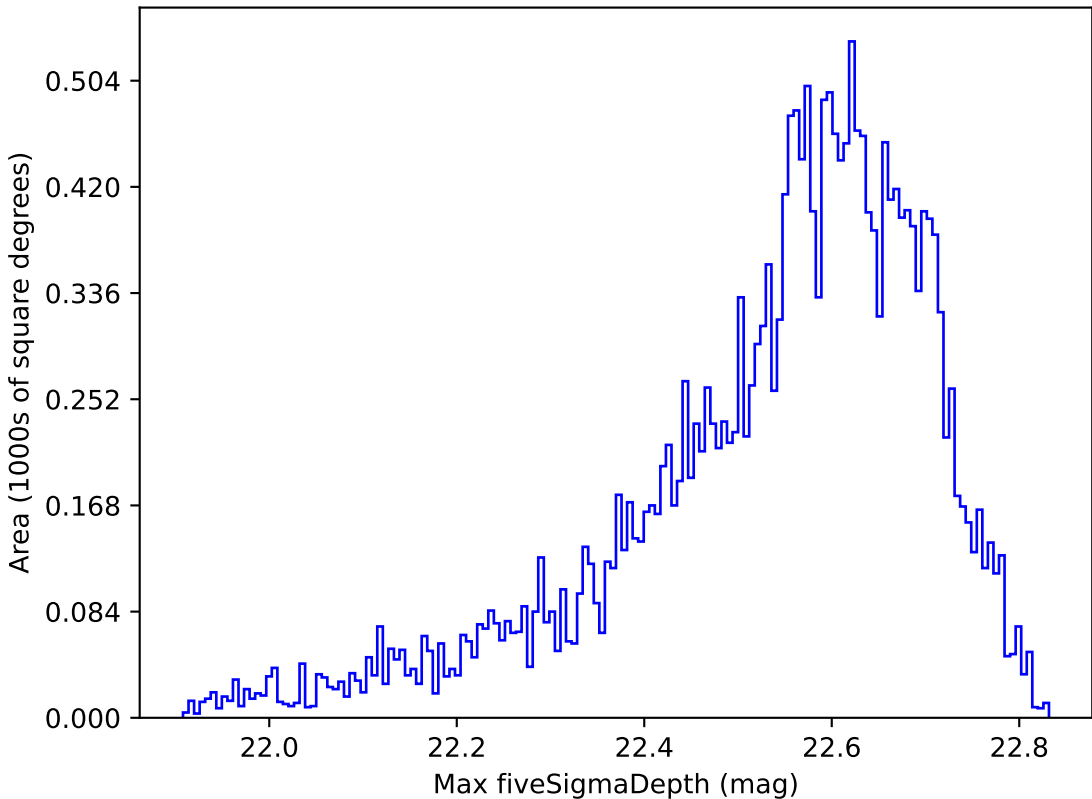
telescope_jerk_v3.5_10yrs All sky y band: Max fiveSigmaDepth
