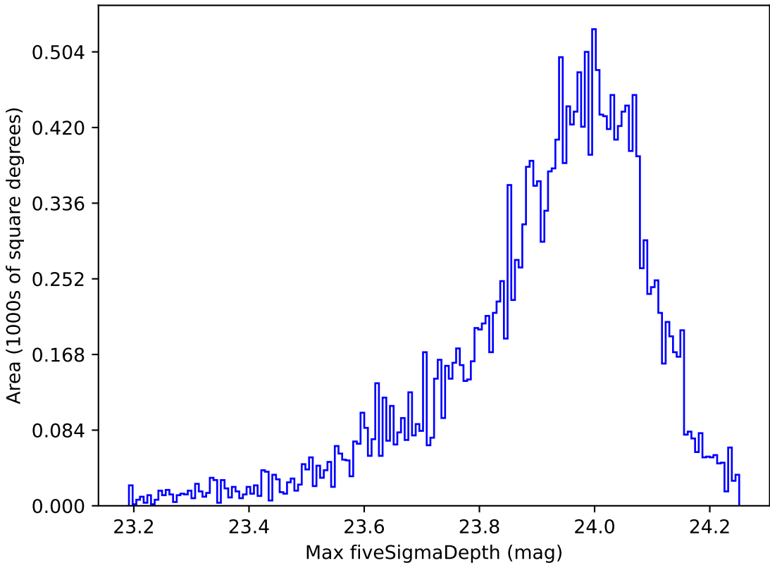
telescope_jerk_v3.5_10yrs All sky u band: Max fiveSigmaDepth
