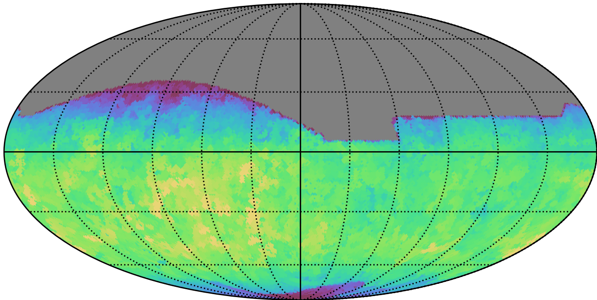
telescope_jerk_v3.5_10yrs All sky r band: Max fiveSigmaDepth
