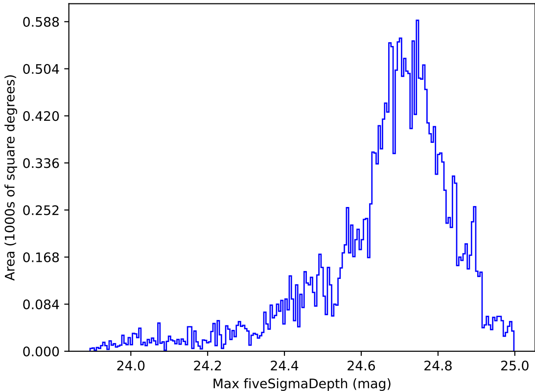
telescope_jerk_v3.5_10yrs All sky r band: Max fiveSigmaDepth
