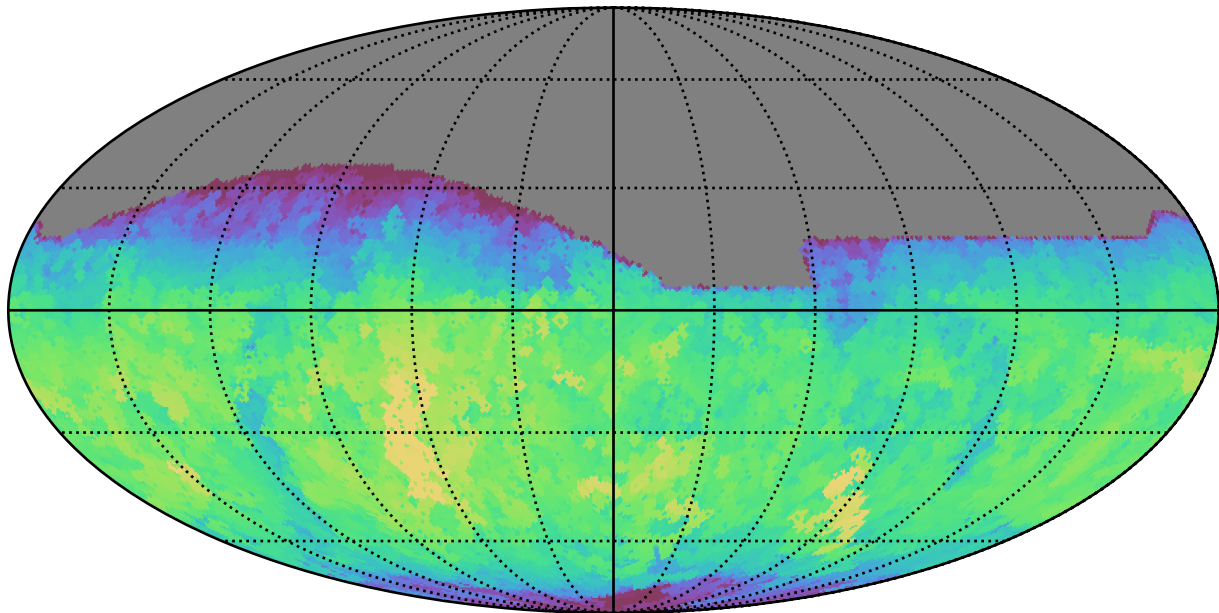
telescope_jerk_v3.5_10yrs All sky i band: Max fiveSigmaDepth
