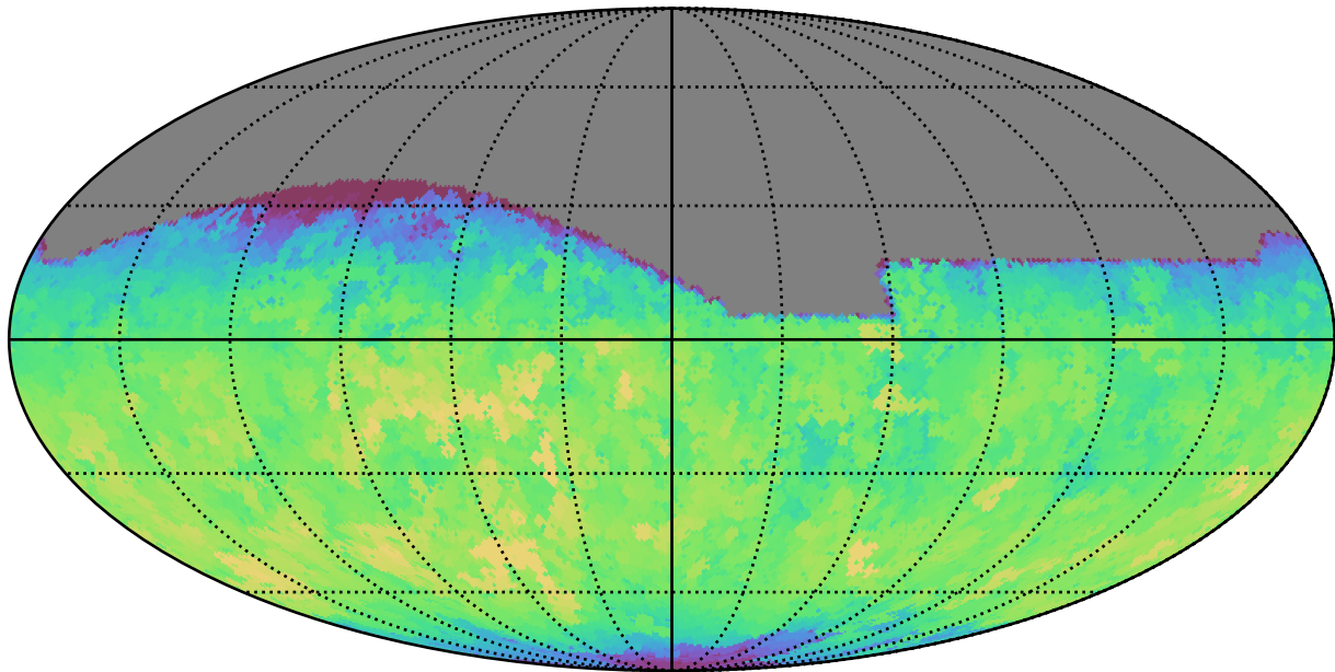
telescope_jerk_v3.5_10yrs All sky g band: Max fiveSigmaDepth
