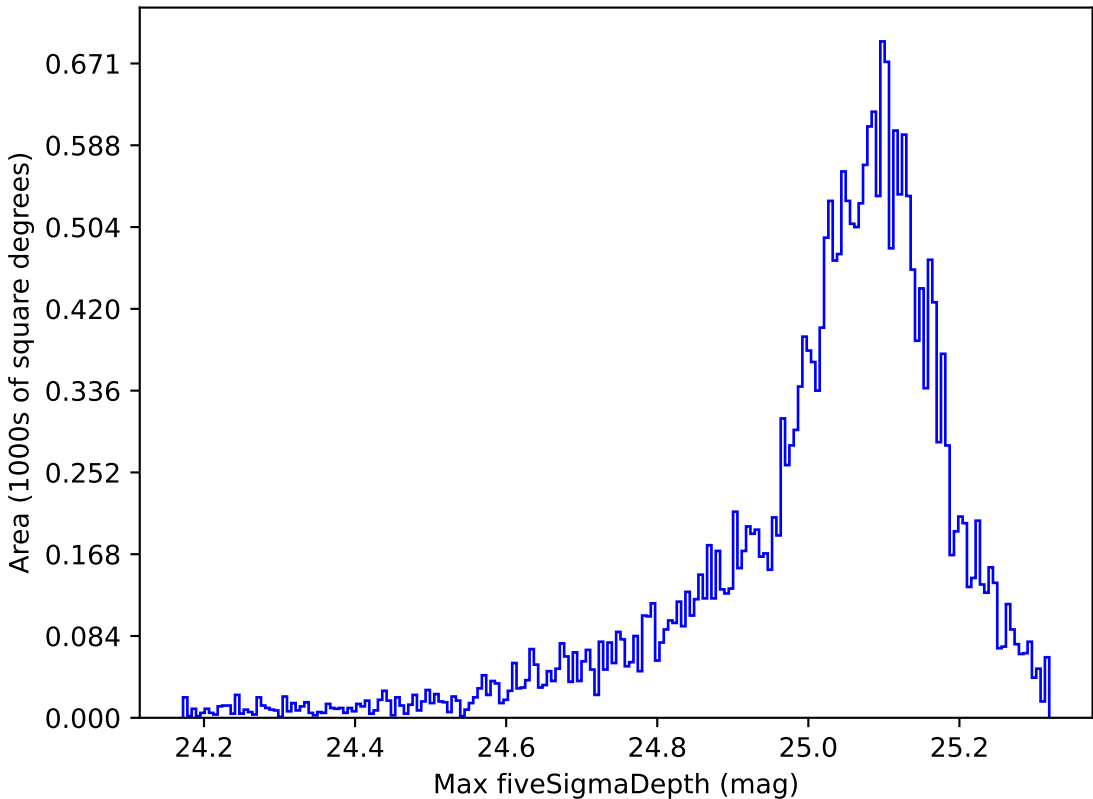
telescope_jerk_v3.5_10yrs All sky g band: Max fiveSigmaDepth
