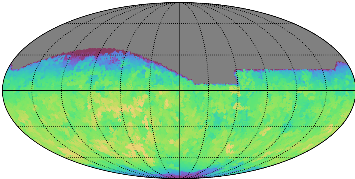
telescope_jerk_v3.5_10yrs All sky all bands: Max fiveSigmaDepth
