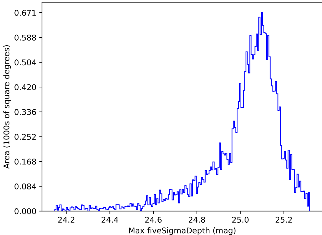
telescope_jerk_v3.5_10yrs All sky all bands: Max fiveSigmaDepth
