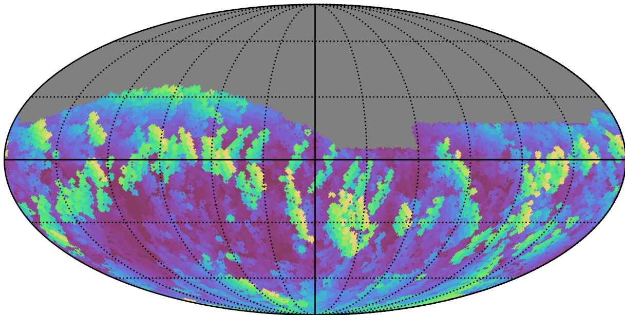
telescope_jerk_v3.5_10yrs Yr 1 z band: Max airmass
