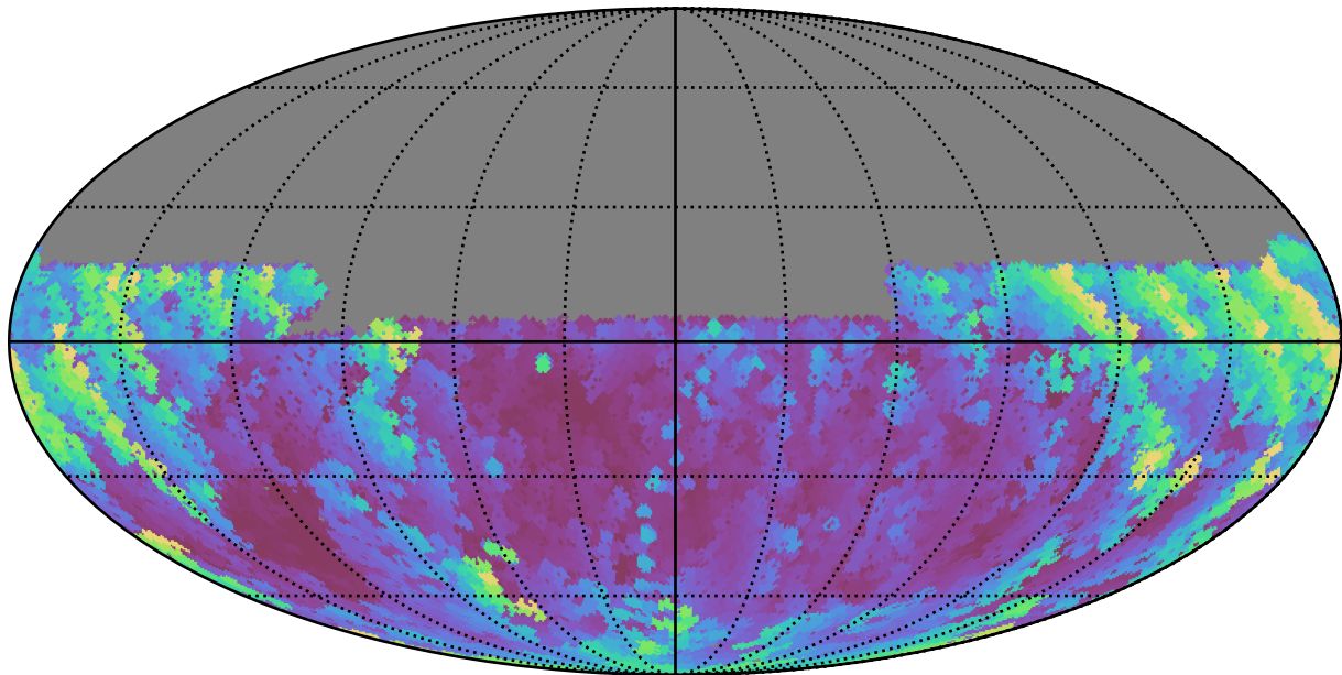
telescope_jerk_v3.5_10yrs Yr 1 y band: Max airmass
