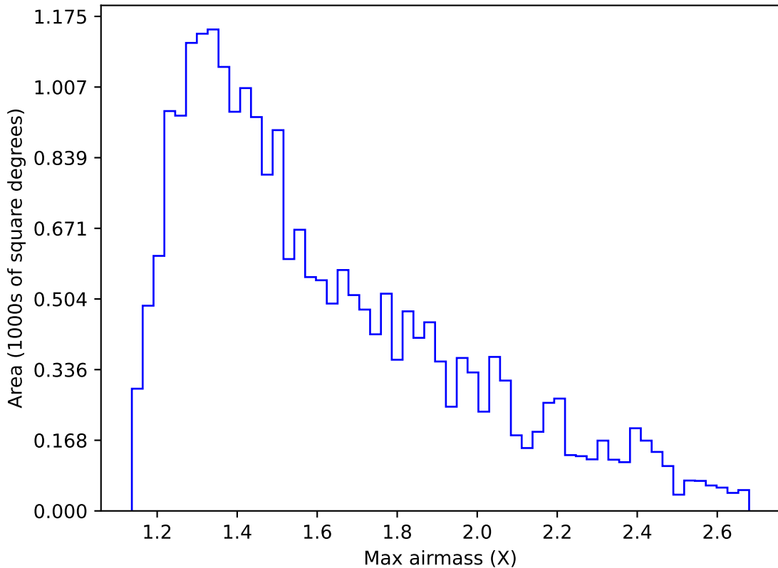
telescope_jerk_v3.5_10yrs Yr 1 y band: Max airmass
