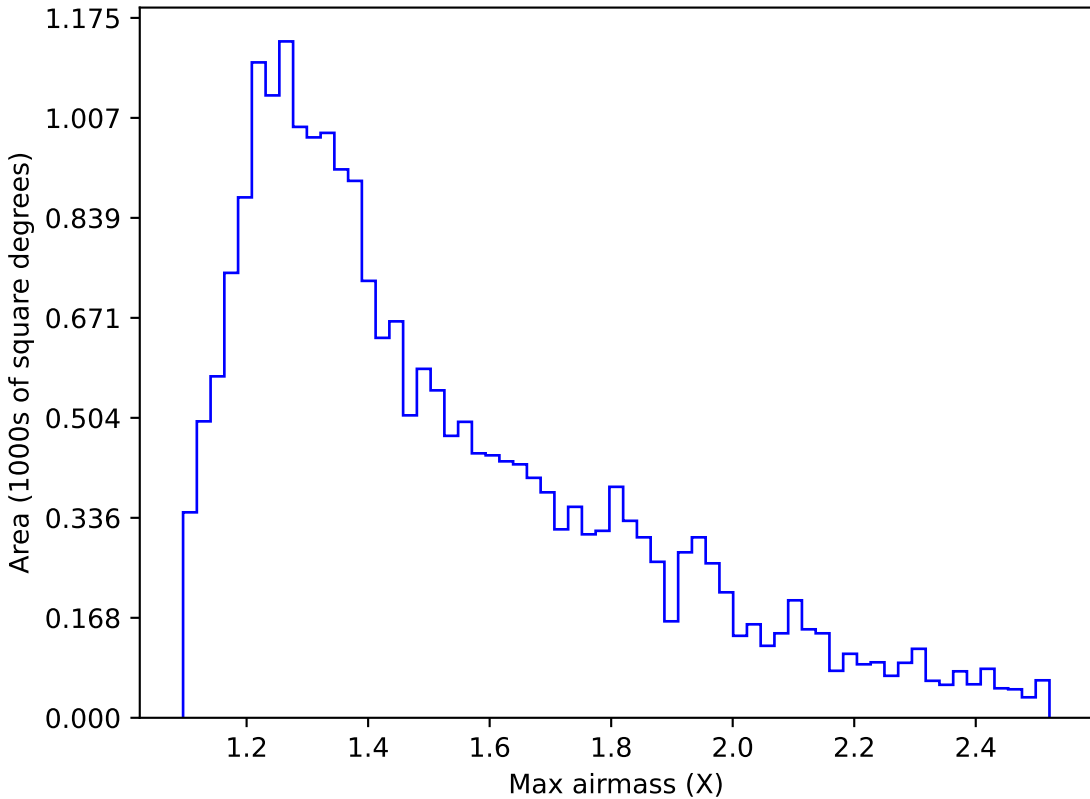
telescope_jerk_v3.5_10yrs Yr 1 u band: Max airmass
