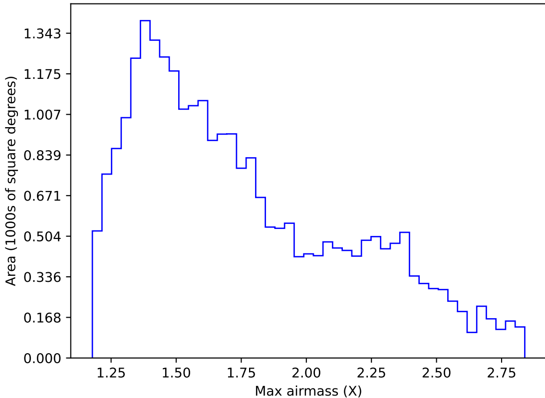
telescope_jerk_v3.5_10yrs Yr 1 r band: Max airmass
