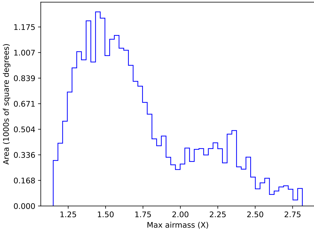
telescope_jerk_v3.5_10yrs Yr 1 i band: Max airmass
