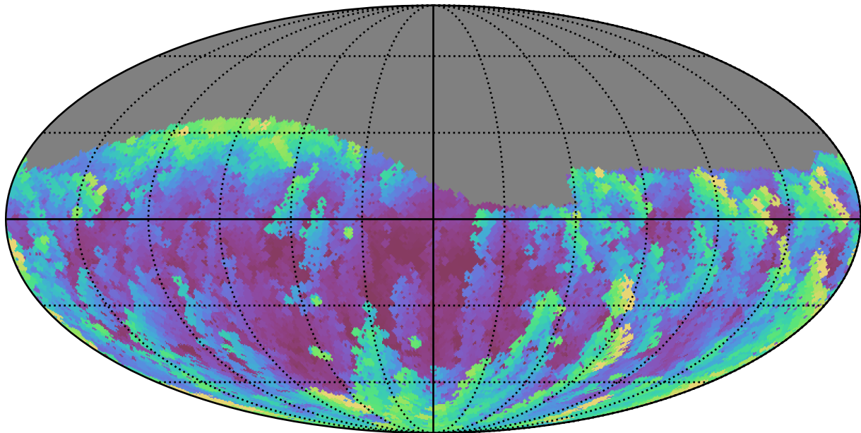
telescope_jerk_v3.5_10yrs Yr 1 g band: Max airmass
