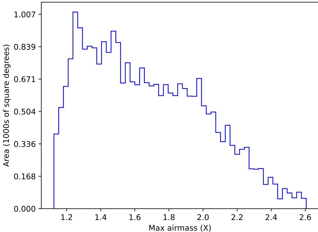
telescope_jerk_v3.5_10yrs Yr 1 g band: Max airmass
