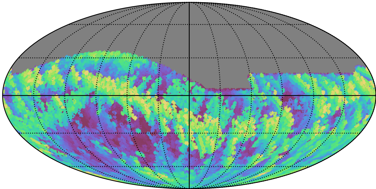
telescope_jerk_v3.5_10yrs Yr 1 all bands: Max airmass
