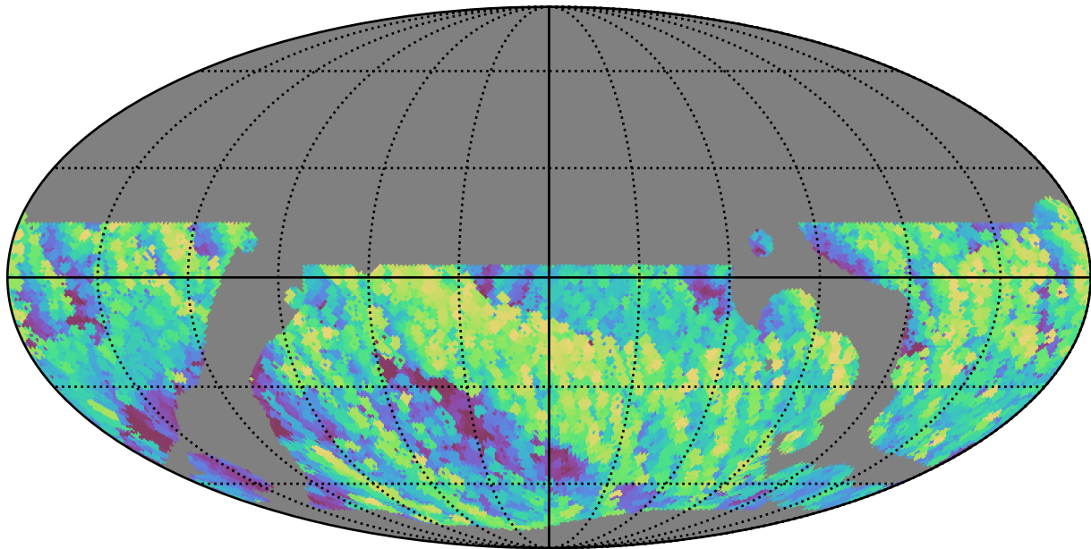
telescope_jerk_v3.5_10yrs WFD z band: Max airmass
