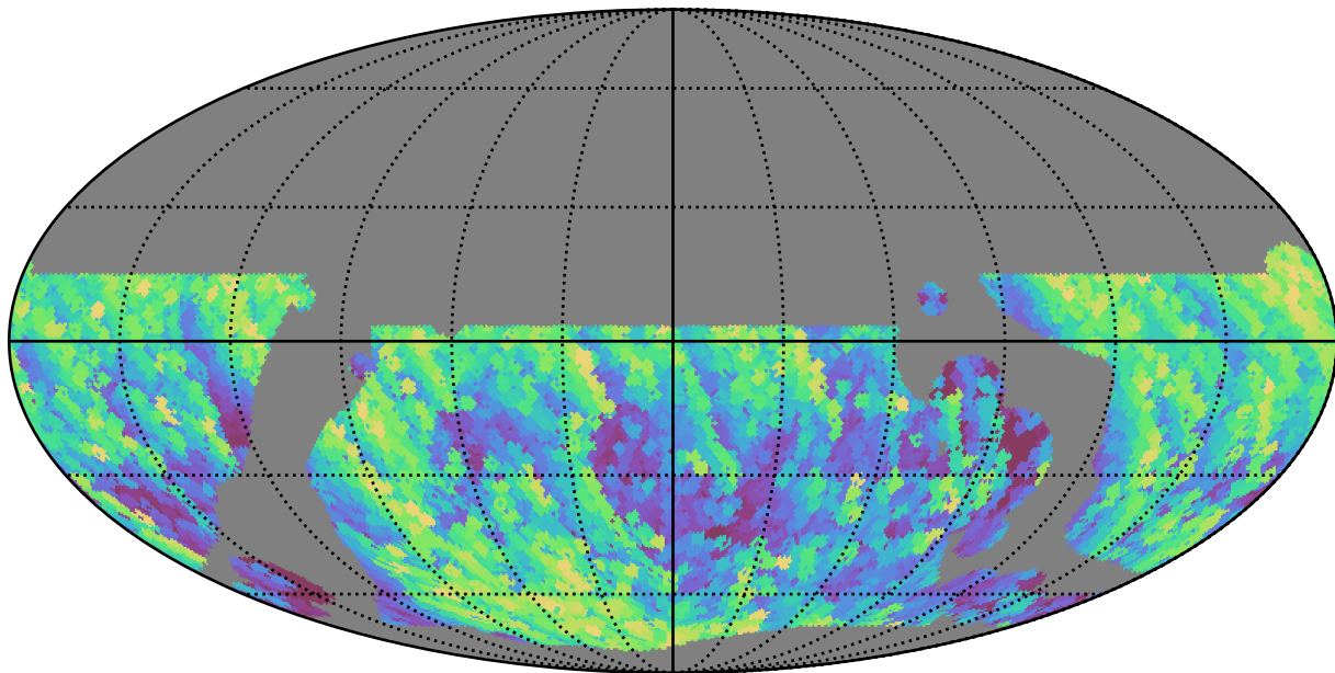
telescope_jerk_v3.5_10yrs WFD y band: Max airmass
