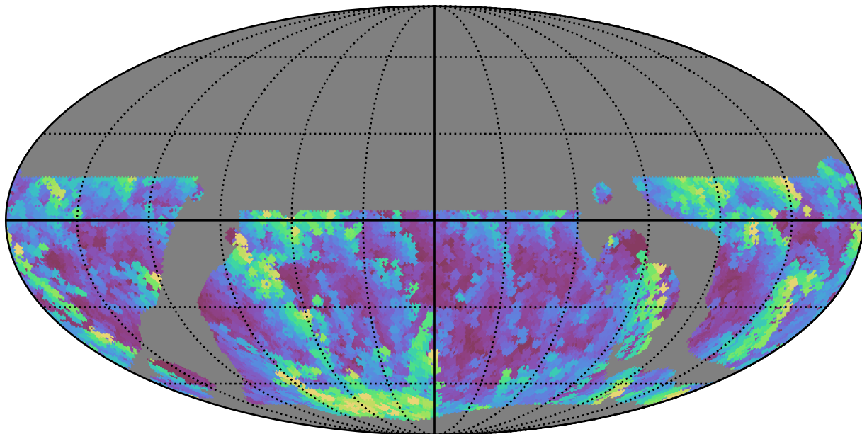
telescope_jerk_v3.5_10yrs WFD u band: Max airmass
