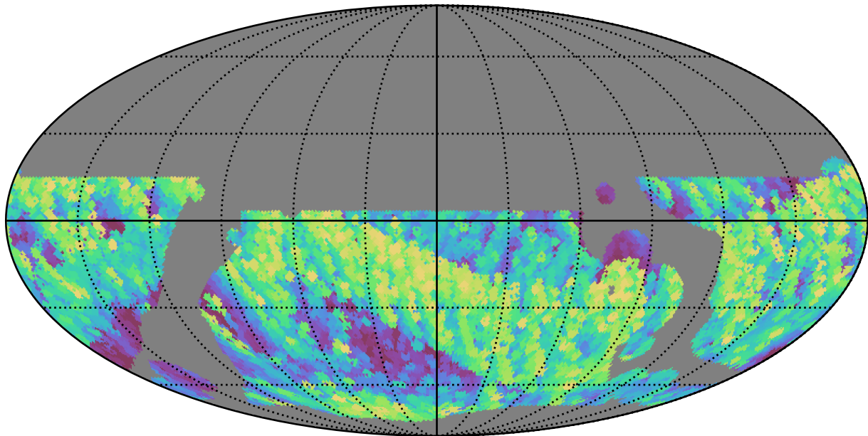
telescope_jerk_v3.5_10yrs WFD i band: Max airmass
