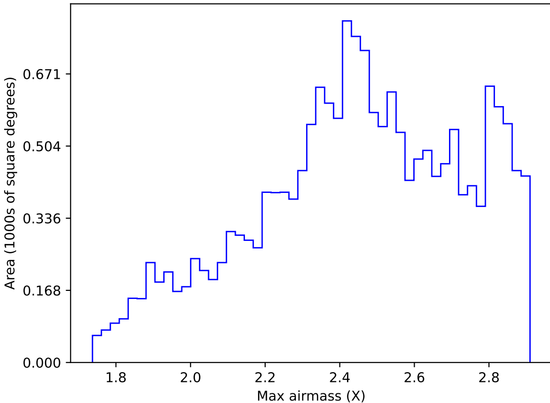
telescope_jerk_v3.5_10yrs WFD i band: Max airmass
