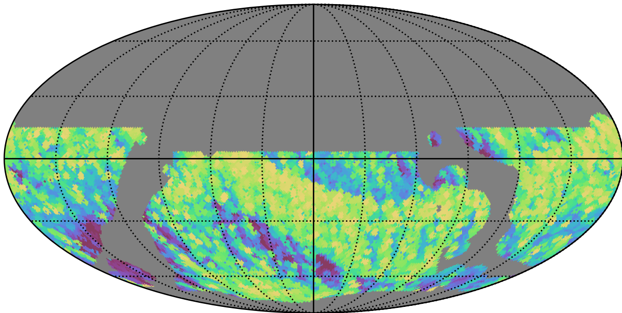
telescope_jerk_v3.5_10yrs WFD all bands: Max airmass
