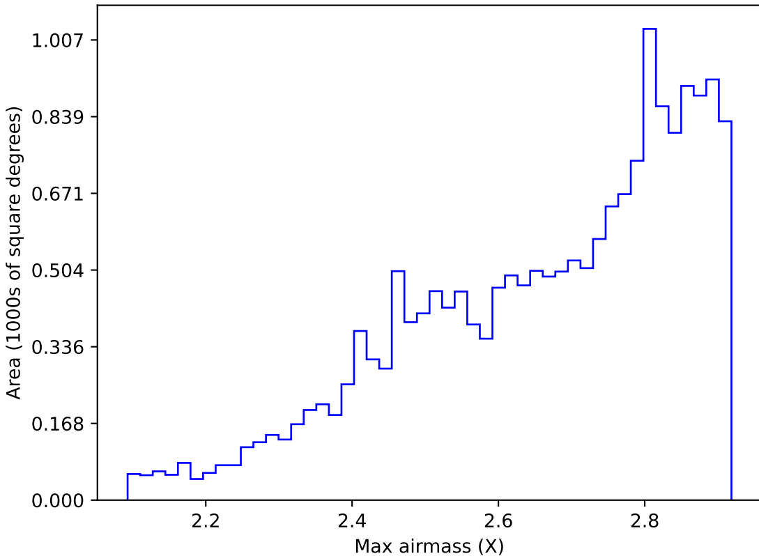
telescope_jerk_v3.5_10yrs WFD all bands: Max airmass
