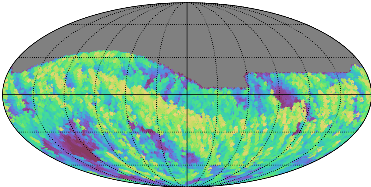
telescope_jerk_v3.5_10yrs All sky z band: Max airmass
