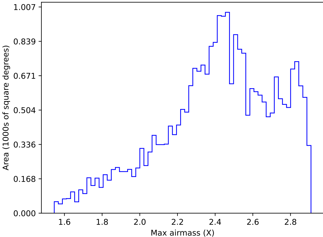
telescope_jerk_v3.5_10yrs All sky z band: Max airmass
