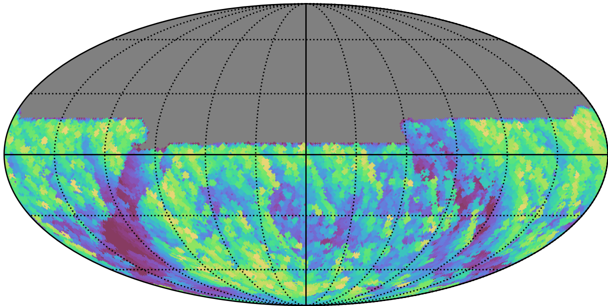
telescope_jerk_v3.5_10yrs All sky y band: Max airmass
