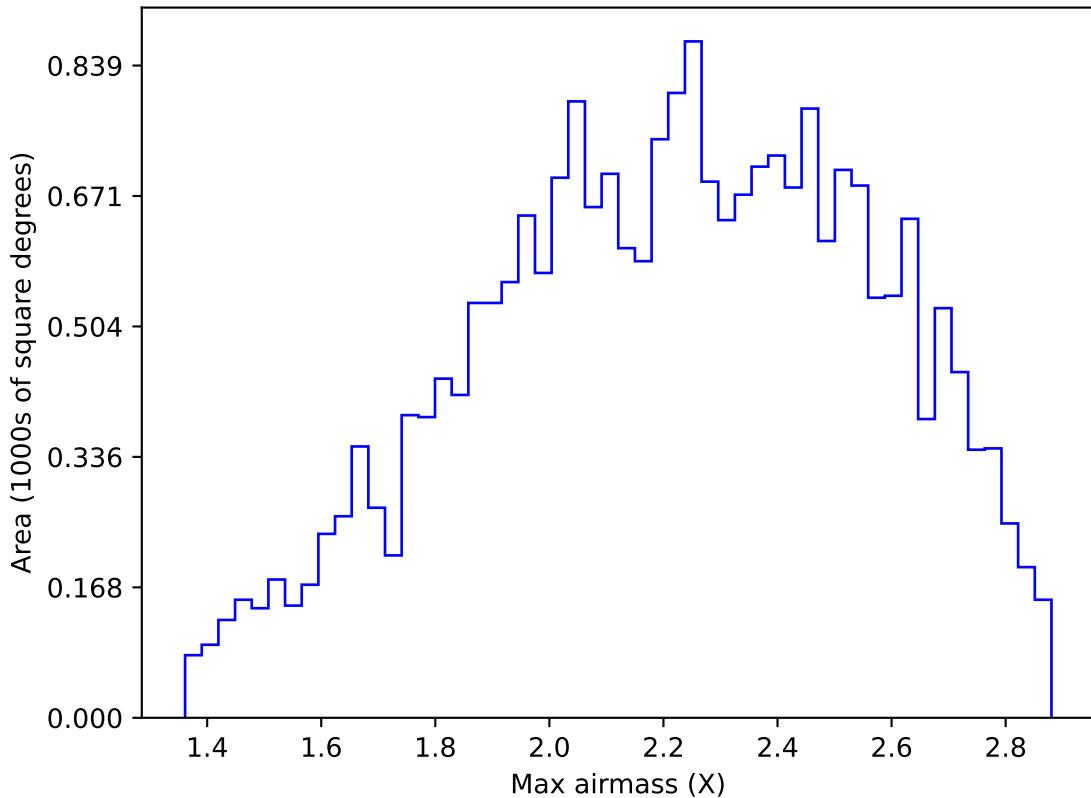
telescope_jerk_v3.5_10yrs All sky y band: Max airmass
