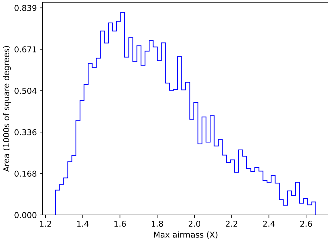
telescope_jerk_v3.5_10yrs All sky u band: Max airmass
