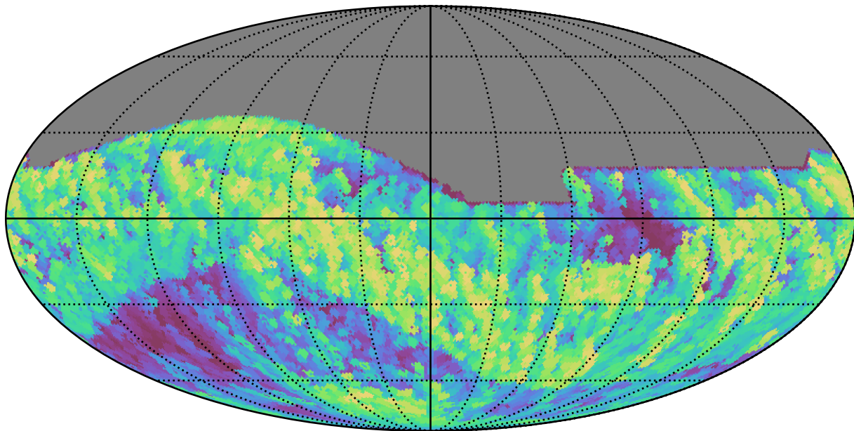
telescope_jerk_v3.5_10yrs All sky r band: Max airmass
