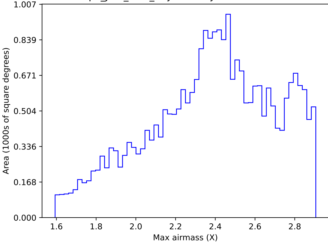
telescope_jerk_v3.5_10yrs All sky r band: Max airmass
