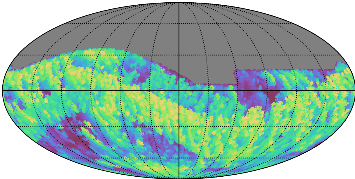
telescope_jerk_v3.5_10yrs All sky i band: Max airmass
