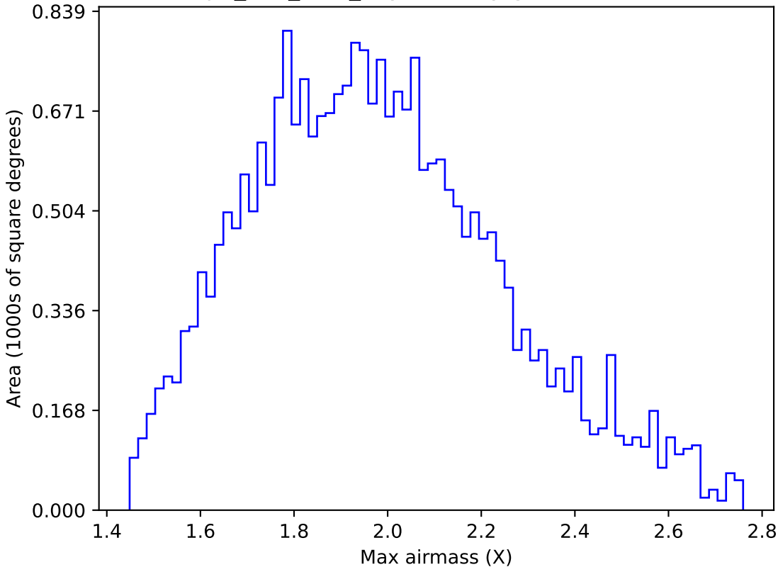
telescope_jerk_v3.5_10yrs All sky g band: Max airmass
