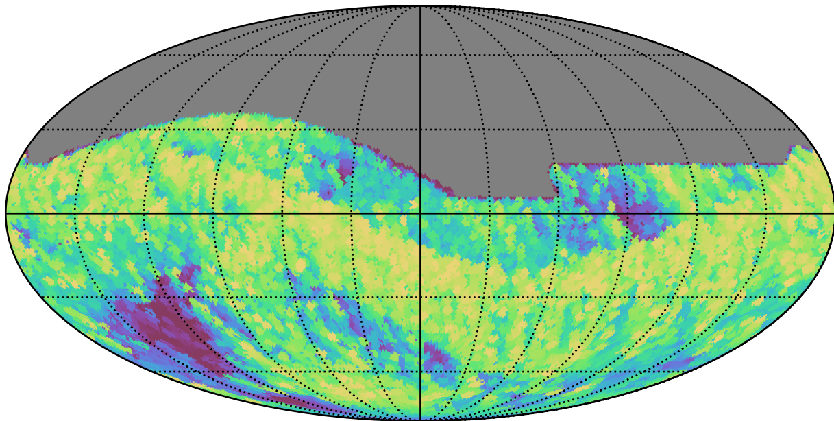
telescope_jerk_v3.5_10yrs All sky all bands: Max airmass
