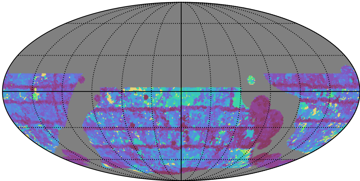
telescope_jerk_v3.5_10yrs WFD z band: Max Inter-Night Gap
