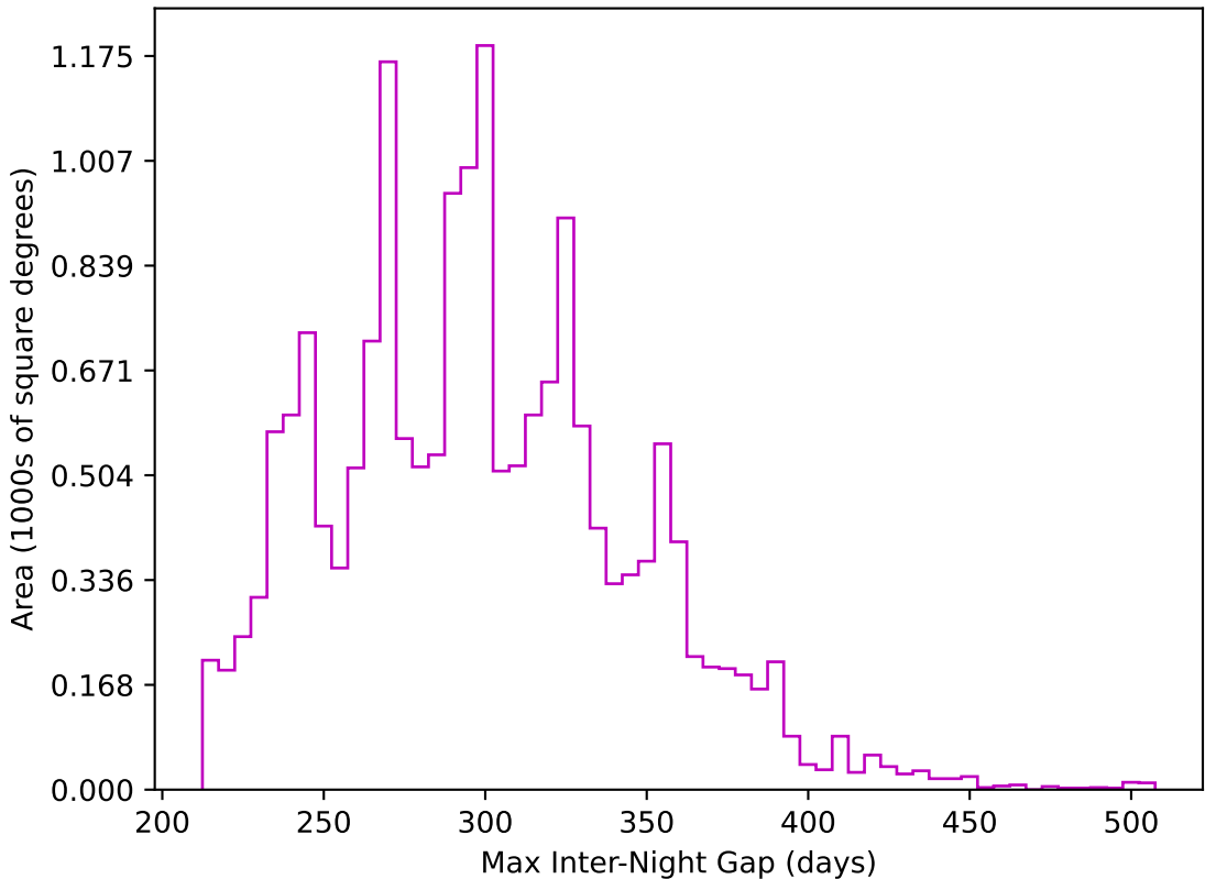
telescope_jerk_v3.5_10yrs WFD z band: Max Inter-Night Gap
