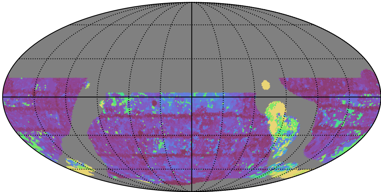
telescope_jerk_v3.5_10yrs WFD y band: Max Inter-Night Gap
