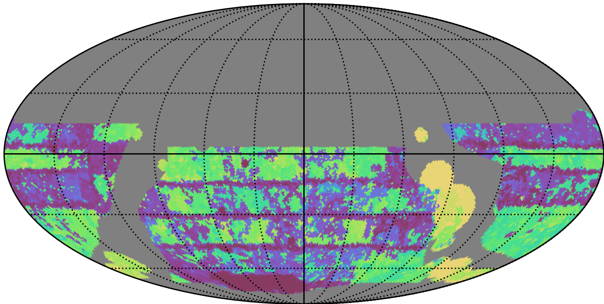
telescope_jerk_v3.5_10yrs WFD u band: Max Inter-Night Gap
