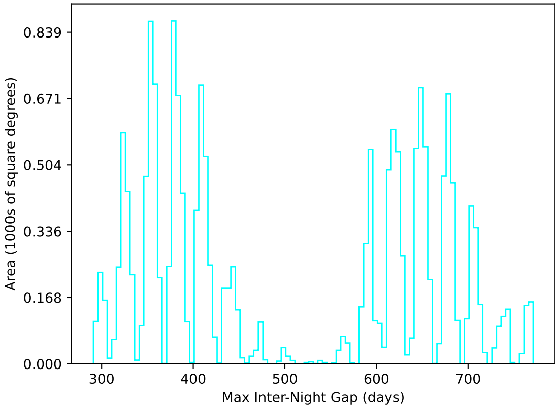
telescope_jerk_v3.5_10yrs WFD u band: Max Inter-Night Gap
