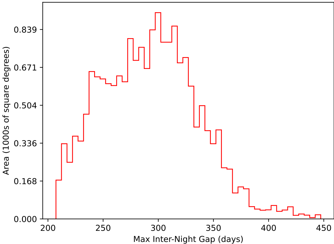
telescope_jerk_v3.5_10yrs WFD i band: Max Inter-Night Gap
