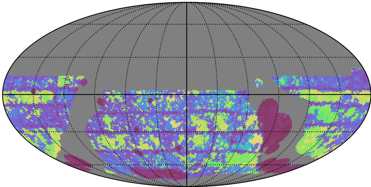
telescope_jerk_v3.5_10yrs WFD g band: Max Inter-Night Gap
