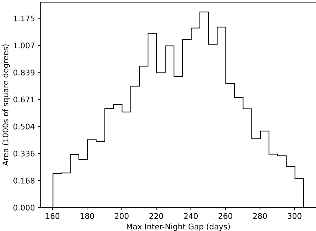
telescope_jerk_v3.5_10yrs WFD all bands: Max Inter-Night Gap
