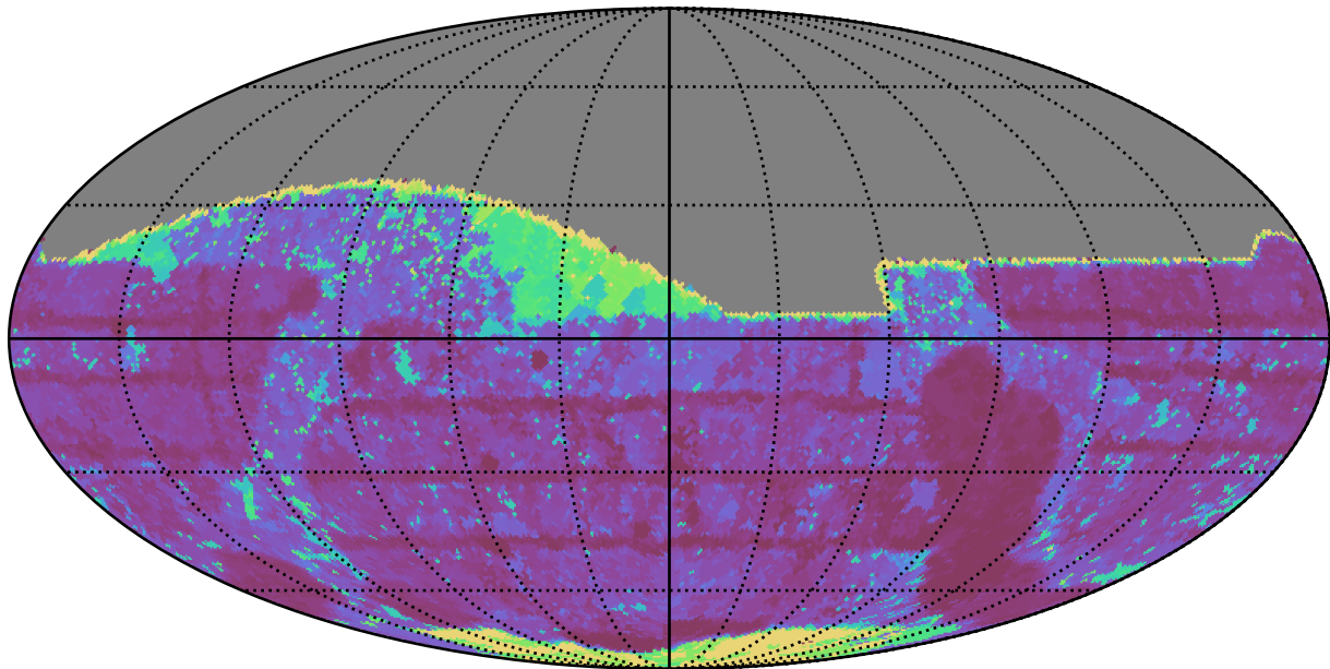
telescope_jerk_v3.5_10yrs All sky z band: Max Inter-Night Gap
