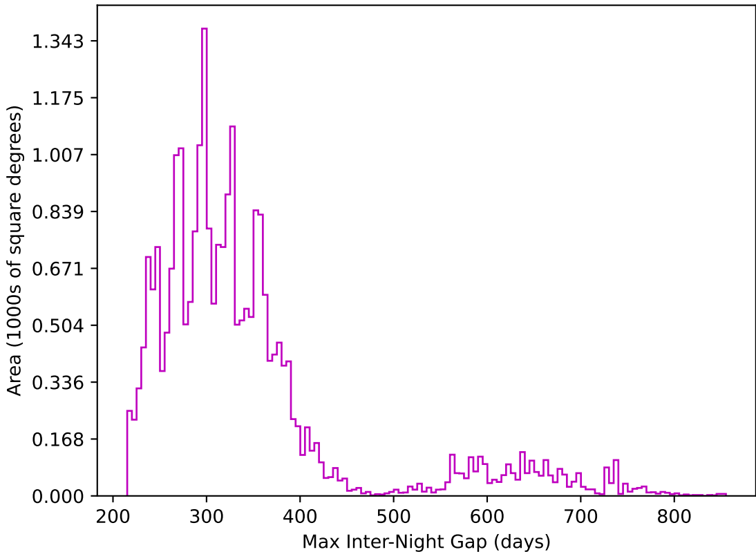
telescope_jerk_v3.5_10yrs All sky z band: Max Inter-Night Gap
