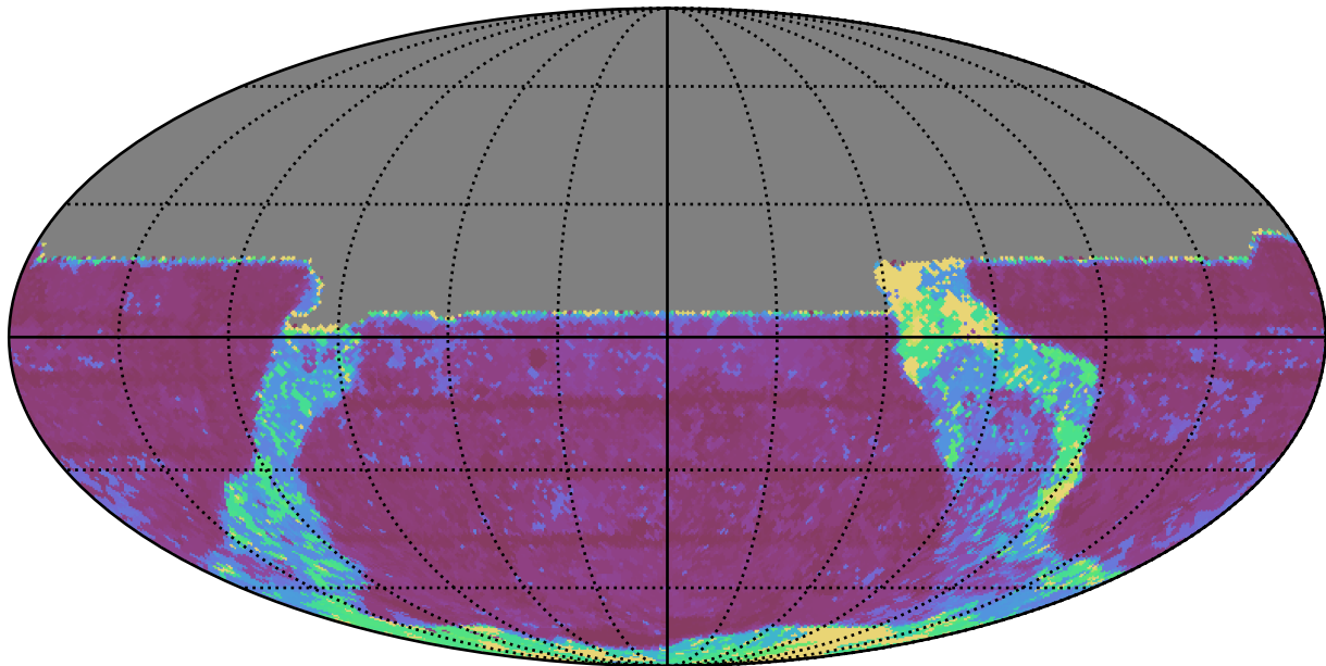
telescope_jerk_v3.5_10yrs All sky y band: Max Inter-Night Gap
